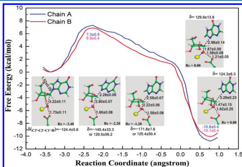
Figure 4. Free energy profiles and the active-site structures along the hydrolysis reaction for Model D.
