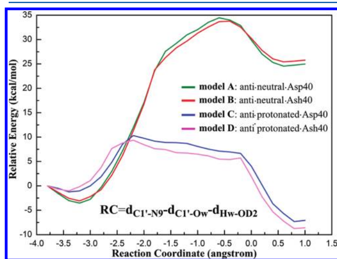
Figure 3. Relative energy profiles along the defined reaction coordinate for various computational models.
