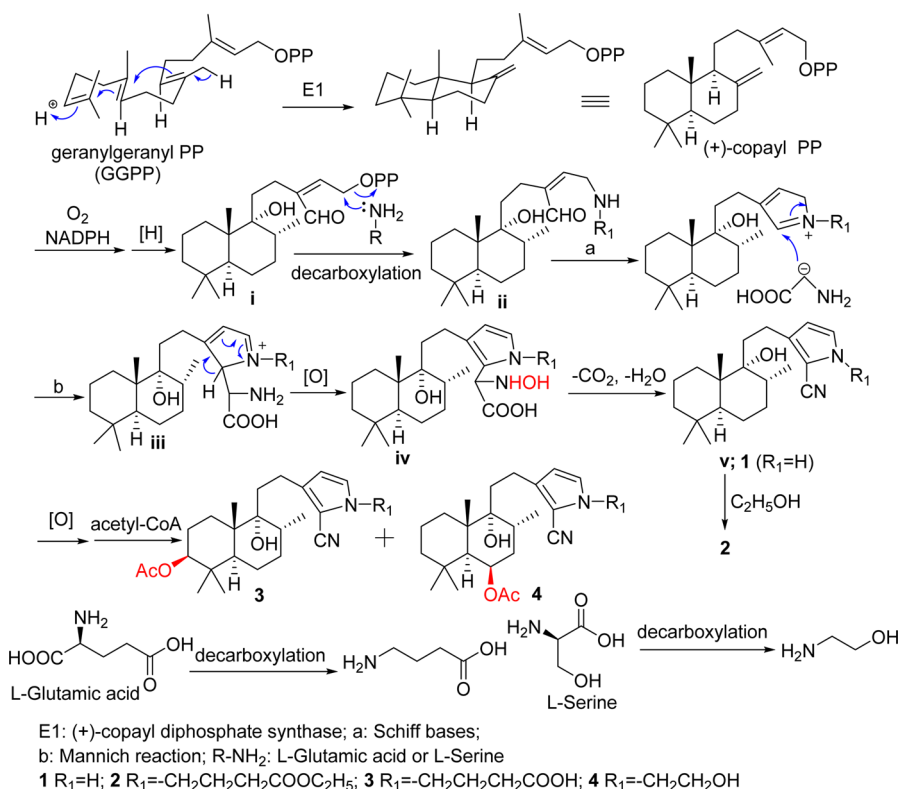
Figure 4. Proposed biosynthetic origin of compounds 1–4.
