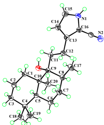
Figure 2. PLATON drawing of compound 1.
